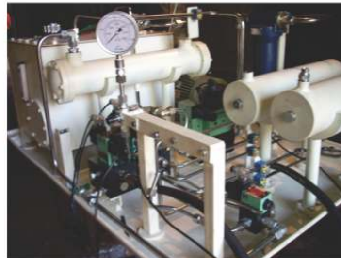
Hyd. System of Tank Transponder
